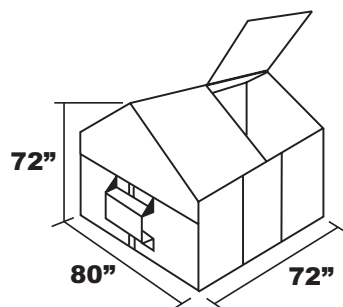
8 Cubic Yard Container
