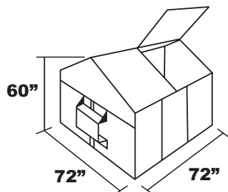
Slant 6 Cubic Yard Container
