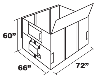
Low Top and Side Loading 6 Cubic Yard Container
